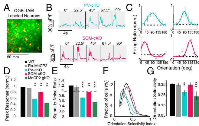
Fig. 3. Deleting MeCP2 results in weak and unselective responses to sinusoidal gratings. (A) Example of an OGB1-AM-labeled population of neurons. Neurons were identified by OGB1 expression (green), whereas astrocytes were identified by SR-101 expression (red). Astrocytes were discarded from further analysis (Materials and Methods). Representative Ca 2+ responses (B) and orientation tuning curves (C) from two neurons from PV-cKO (Top) and SOM-cKO (Bottom) mice. The Ca 2+ responses correspond to the leftmost tuning curves in C. Error bars represent SEM across 10 repeats of each orientation. deg, degrees; \Delta F/F , changes in fluorescence activity. Normalized peak response (D) and signal-to-noise ratio (E) at the preferred orientation for each of the five experimental conditions are shown. Histogram (F) and normalized OSI (G) values for the five different experimental conditions are shown. Bar colors denote experimental conditions as labeled in D. Data are averaged from WT (327 neurons from six mice), flx-MeCP2 (270 neurons from six mice), PV-cKO (146 neurons from four mice), SOM-cKO (240 neurons from four mice), and MeCP2 gKO (163 neurons from four mice) animals. Error bars denote SEM. * P < 0.05, ** P < 0.01, *** P < 0.001; Kruskal-Wallis ANOVA followed by post hoc Bonferroni-corrected rank-sum tests relative to WT.
